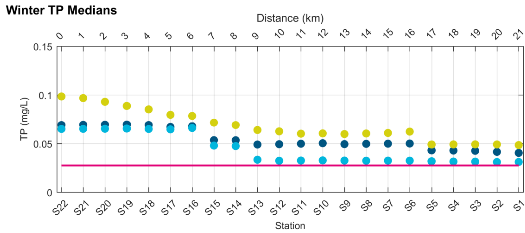
Figure 14 - Total Phosphorous - winter
