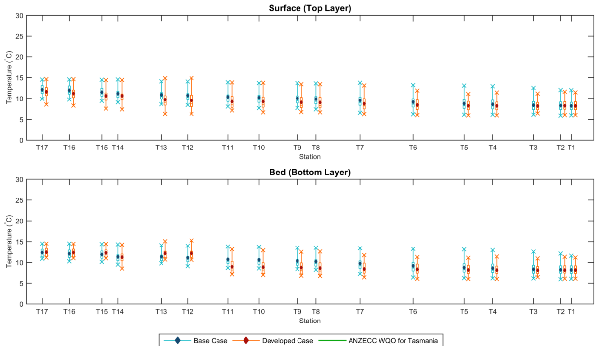
Figure 20 - Water Temperature - summer
