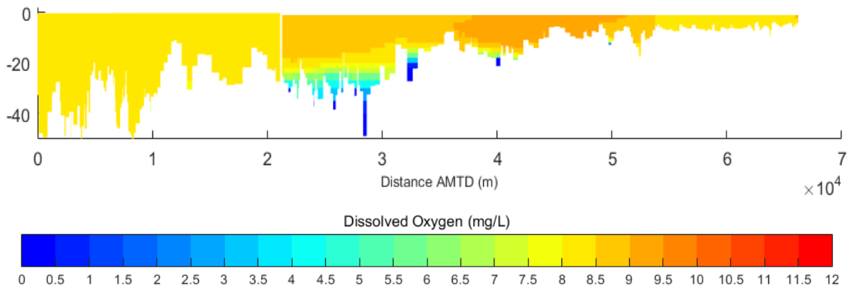
Figure 22 - graphical results of barrage operating strategies
