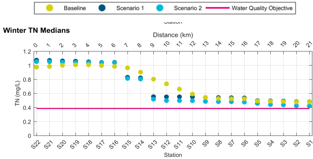
Figure 13 - Total Nitrogen - winter
