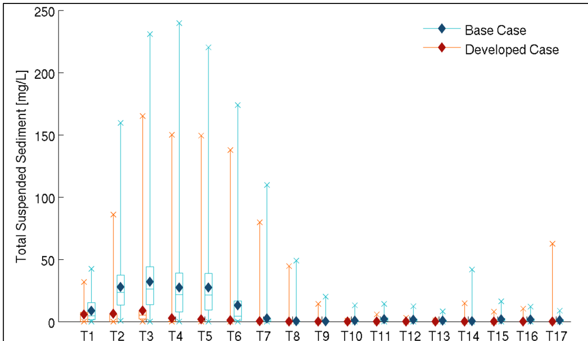
Figure 10 – Modelled Water Turbidity
